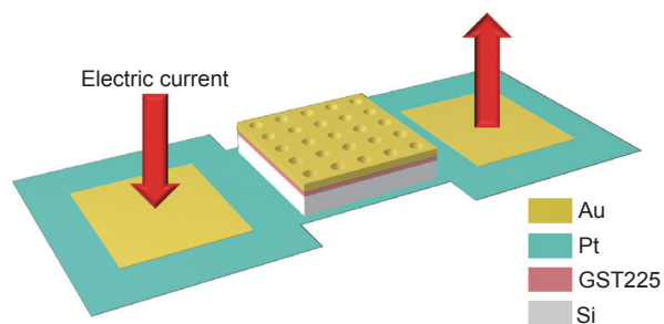
Fig. S2 | Schematic of electrically tuned chalcogenide metamaterials residing on a metallic heater.
