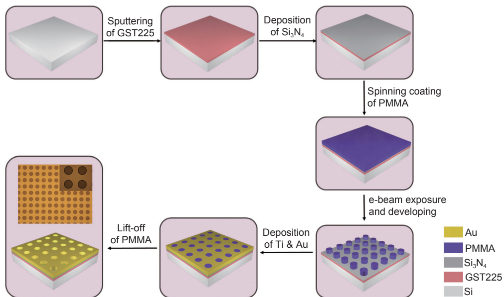
Fig. S1 | The schematic of fabrication processing of the metamaterial.
